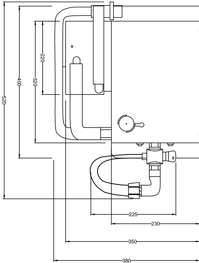
TOP VIEW (Including Mounting Bracket)
