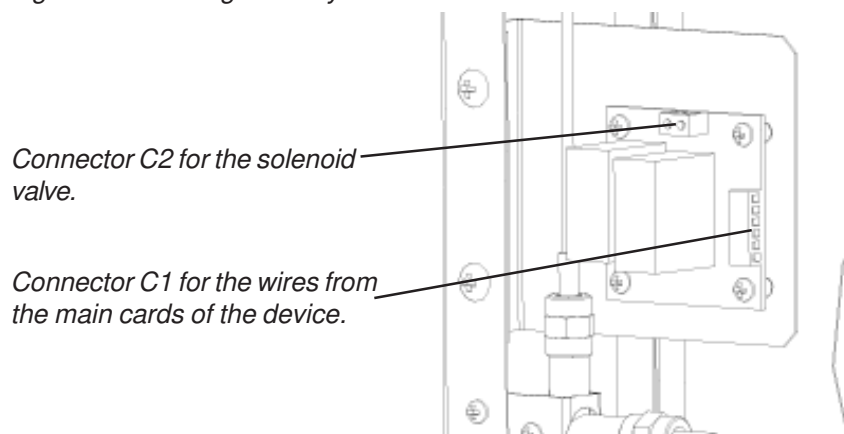
Figure 4: Fastening the relay card and solenoid valve to the stove-oven.
